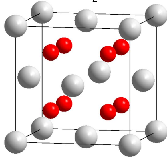
\text{CaF}_2
